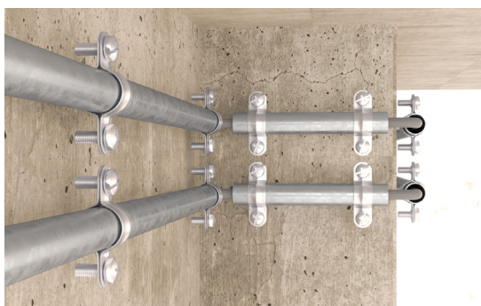
Fixing of empty metal pipes
